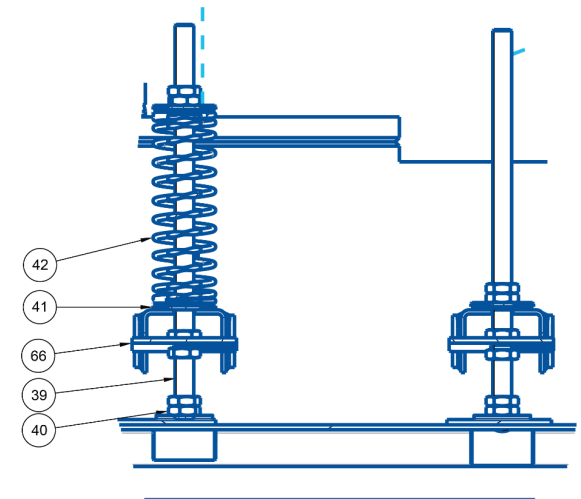
DETAIL VIEW BELT TENSIONER ASSEMBLY
