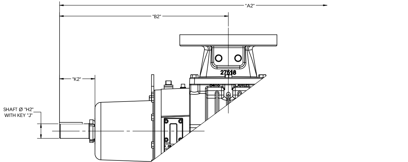
3206 LEFT/RIGHT DRIVE, "DOUBLE-ENVELOPE" MECH SEAL UNIT SHOWN UNLESS OTHERWISE SPECIFIED, ALL DIMENSIONS MATCH THE SINGLE ENV / LIP SEAL UNIT, BELOW
