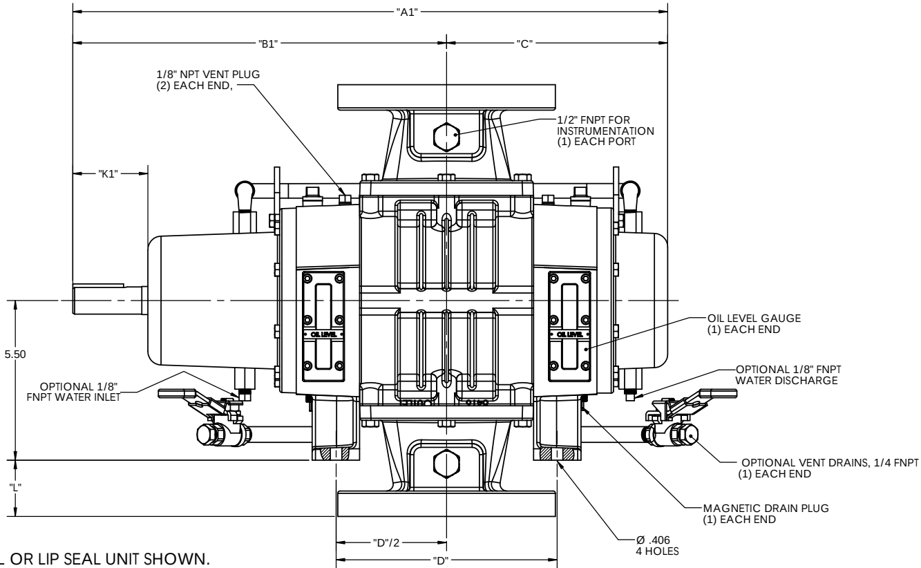
3206 LEFT DRIVE "SINGLE ENVELOPE" MECH SEAL OR LIP SEAL UNIT SHOWN. RIGHT DRIVE SIMILAR. SEE TABLE FOR MODELS WITH DIFFERING LENGTHS
